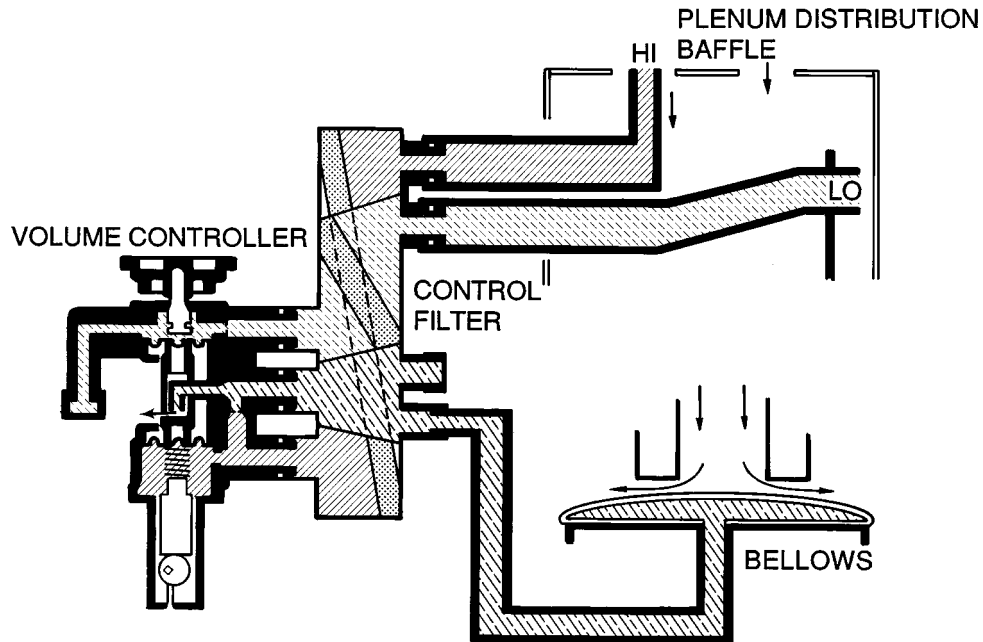
Fig. 54 — Constant Volume Controls — Controller Bleeding, Unit Supplying Air
